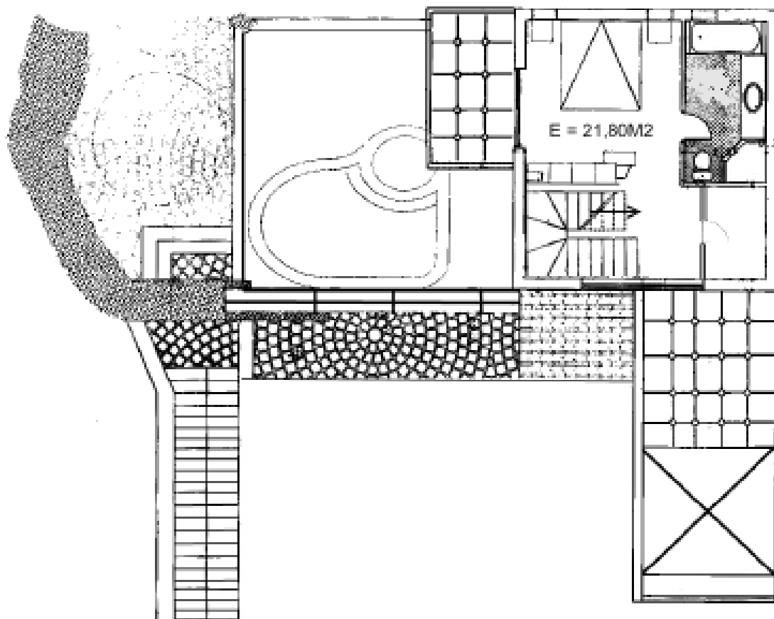
first floor Area: 21.60 m 2
